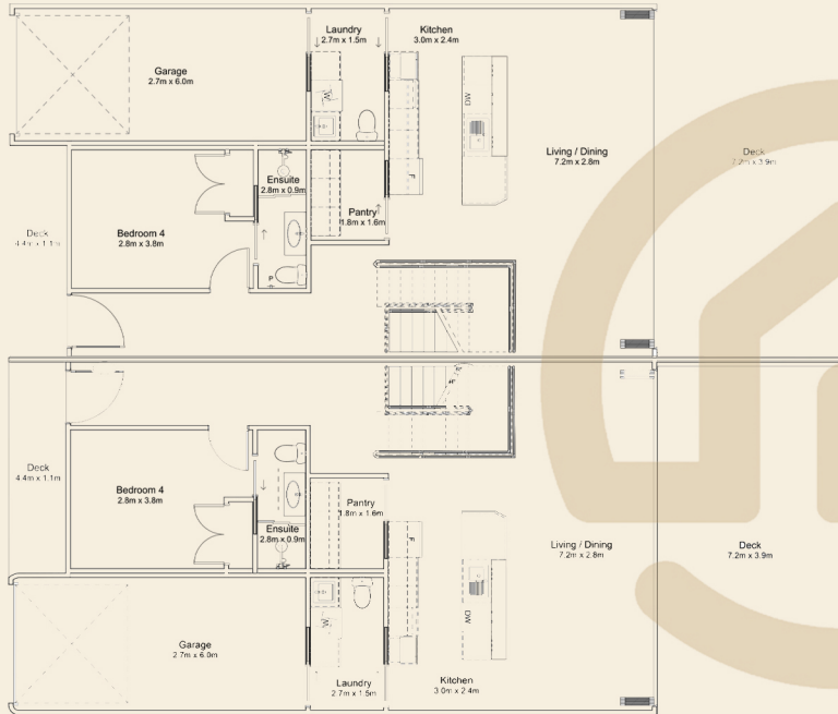
BOTTOM LEVEL
